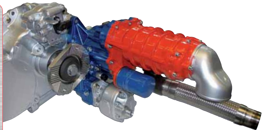
Model with hydraulic pump
